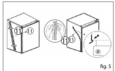
Fig. 5 - Fitting the spacer piece Take out the spacer piece (11) located on the side panel and remove the protective tape. Stick the spacer piece on the opposite side to the door hinges of the appliance.
